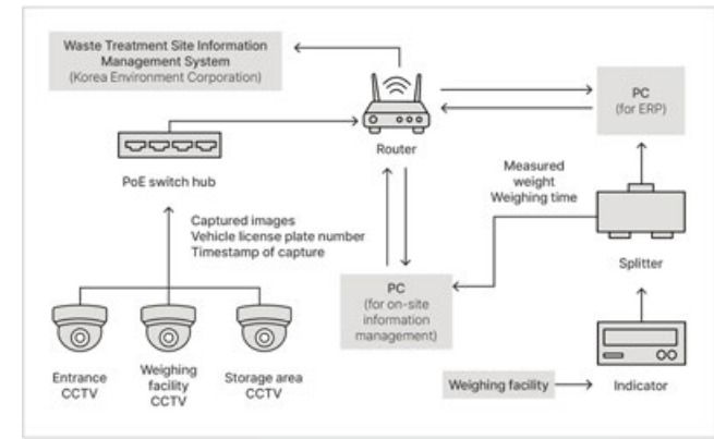
Waste Treatment Site Information System Diagram
